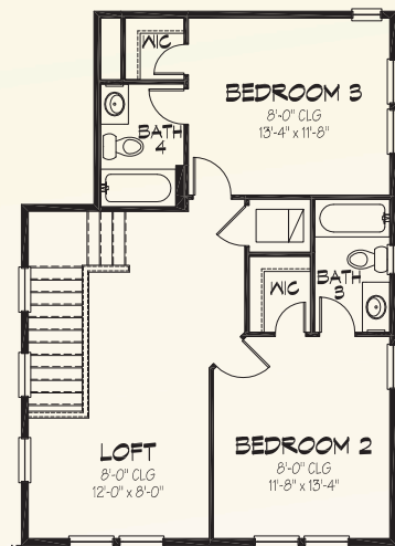
2ND FLOOR PLAN A
