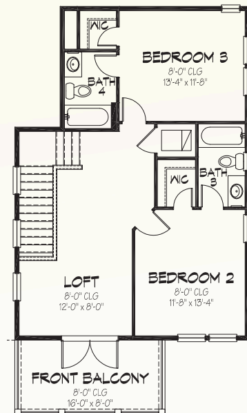
2ND FLOOR PLAN B
